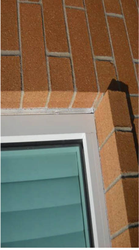
Health Education Building – Typical sealant joint is at end of life.
